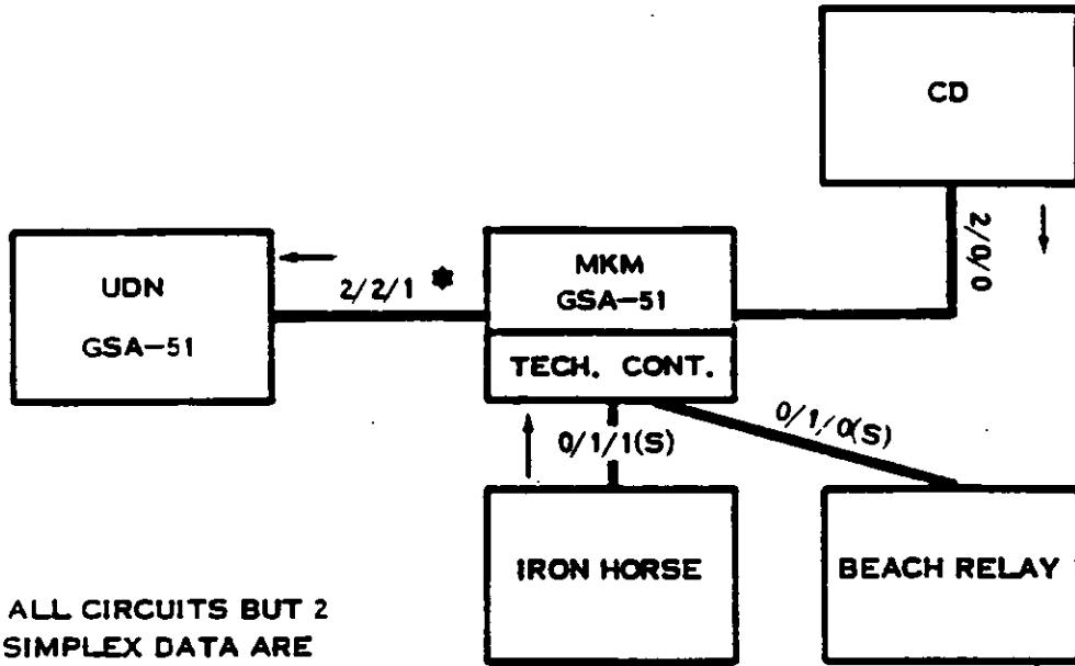
SEEK DAWN PHASE III RECONFIGURATION
