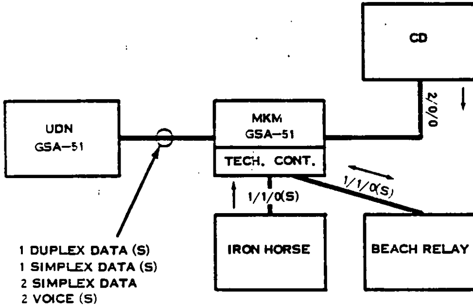
SEEK DAWN PHASE IV RECONFIGURATION
