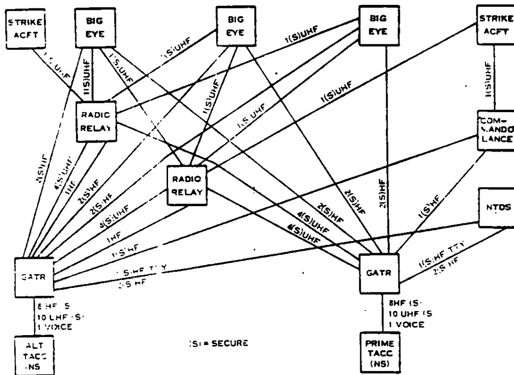
SUMMARY OF RADIO COMMUNICATION REQUIREMENTS
