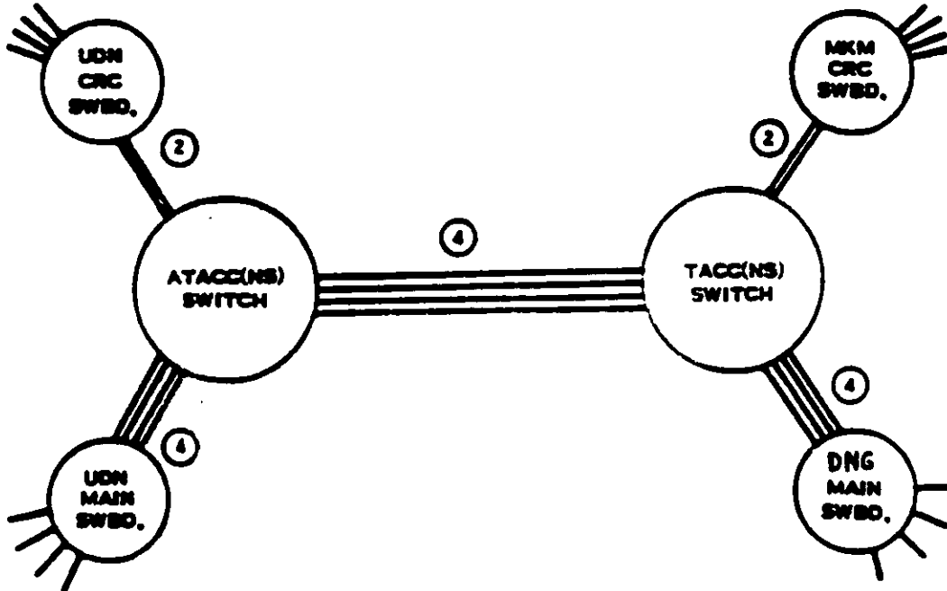
TACC(NS)/ATACC(NS) SWITCH TRUNK TIES
